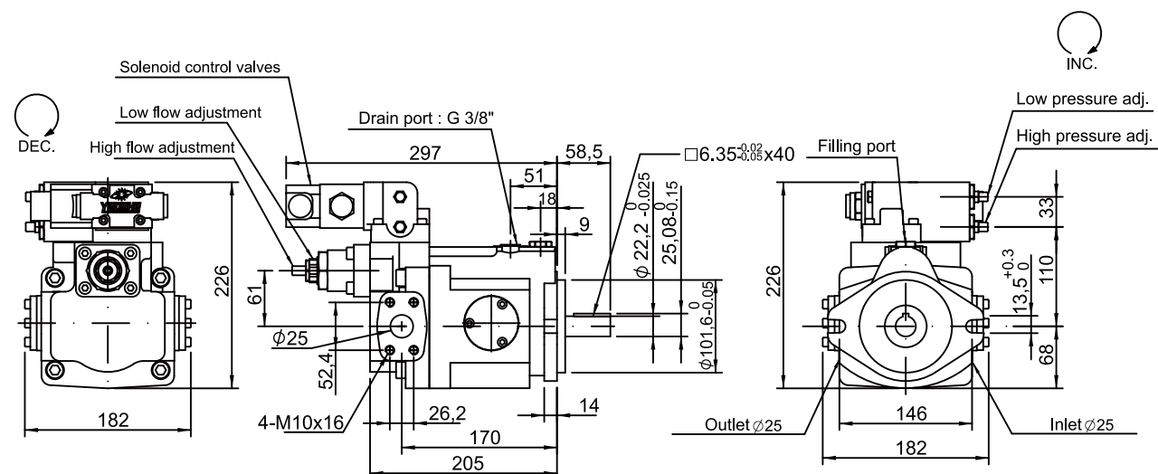
V23F, V25F Electric 2-stage pressure control & Flow control
