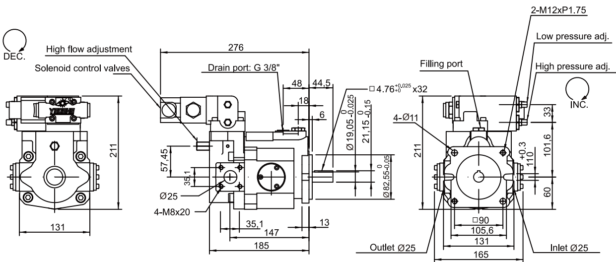
V15D, V18D Low tension unloading + Pressure control
