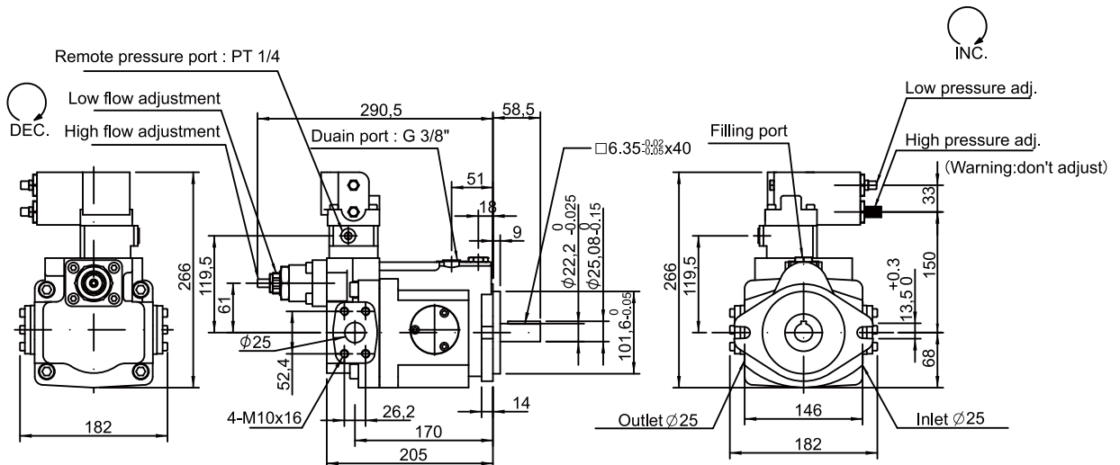
V23CG, V25CG 2-stage pressure & Flow control + Remote
