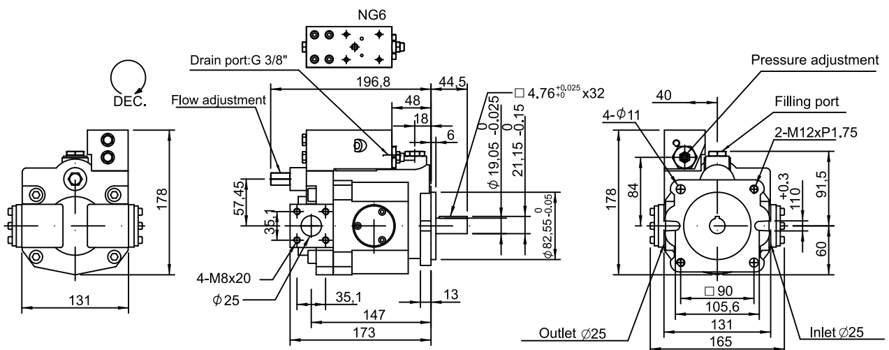
V15GM, V18GM Remote pressure compensator with NG6 interface
