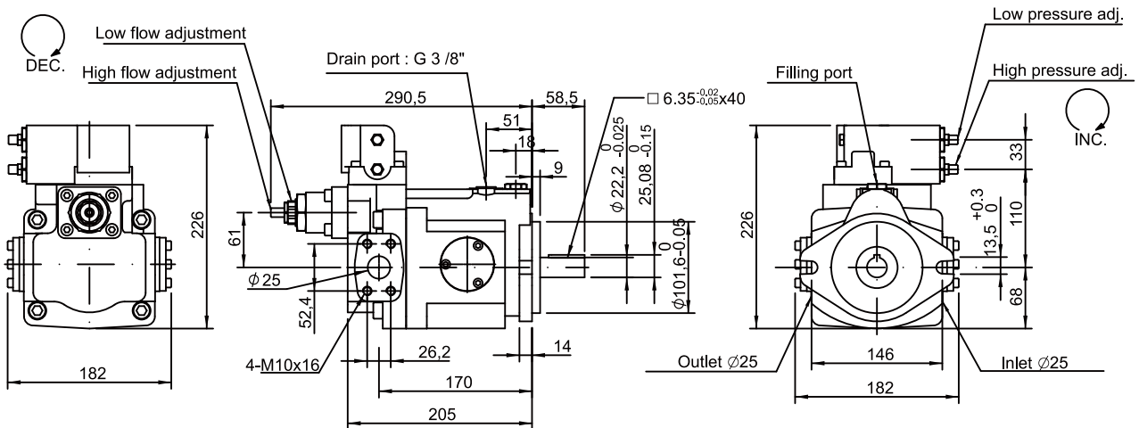
V23C, V25C 2-stage pressure & Flow control
