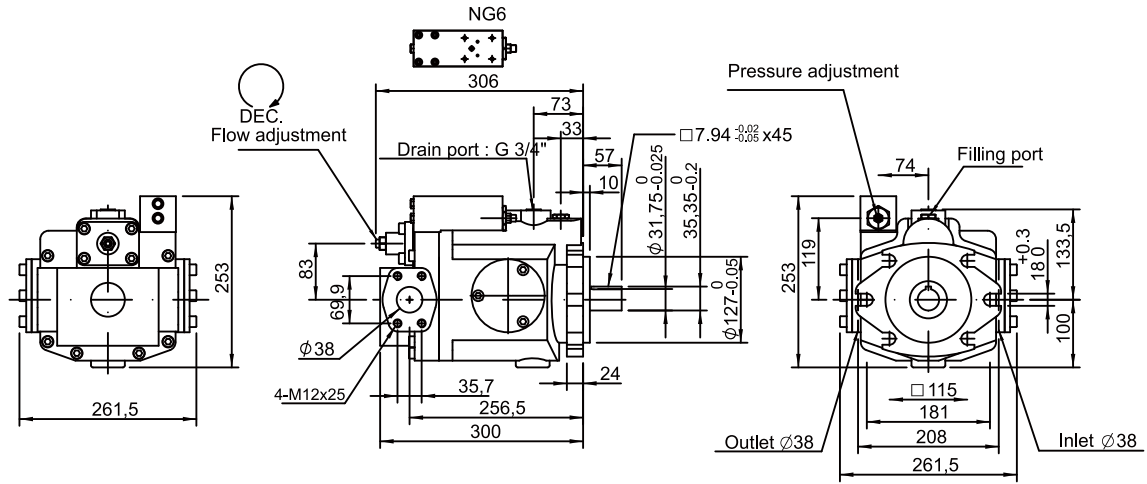
V50GJ, V70GJ Remote pressure compensator + Proportional pressure valve
