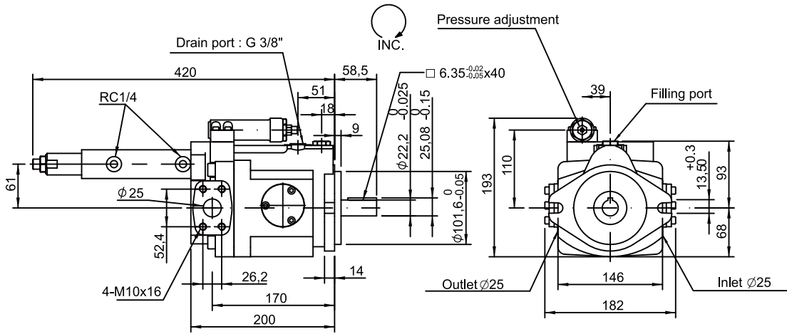
V23C, V25C 2-stage pressure & Flow control
