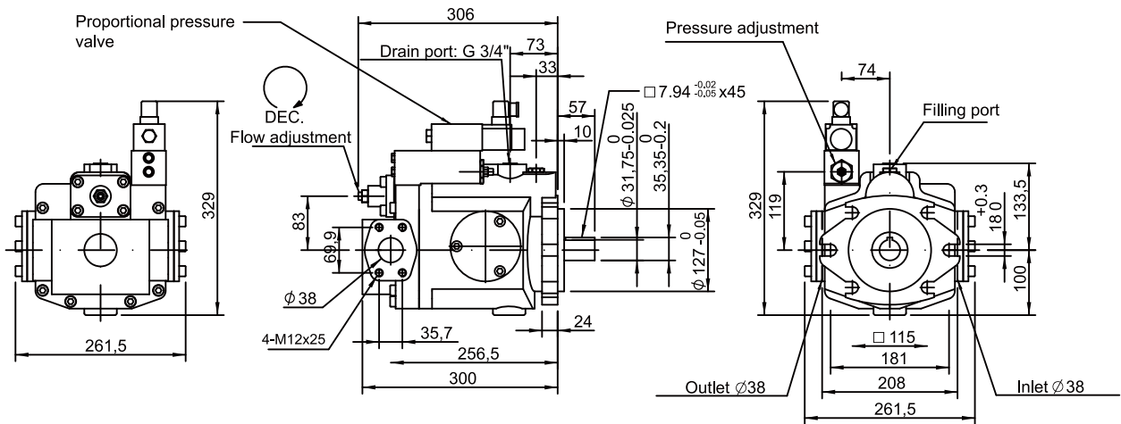
V50GR, V70GR Remote pressure compensator + Electrical unloading
