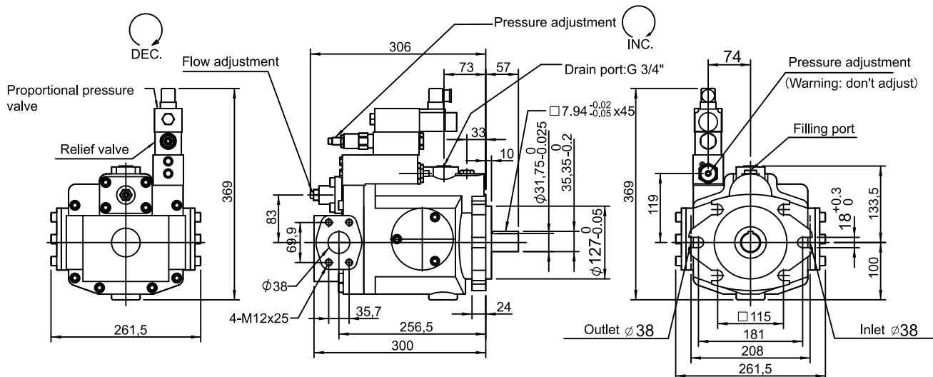
V50GR, V70GR Remote pressure compensator + Electrical unloading
