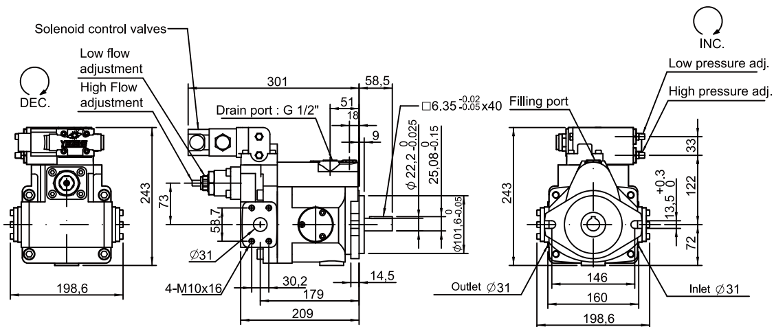
V38F, V42F Electric 2-stage pressure control & Flow control
