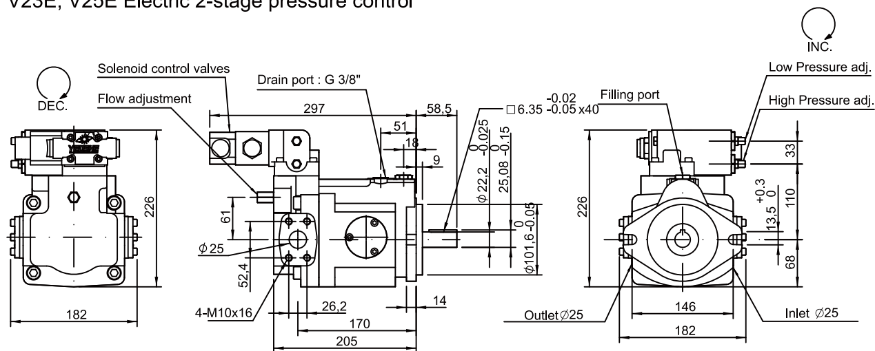
V23E, V25E Electric 2-stage pressure control
