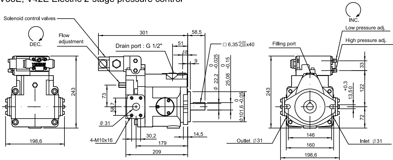
V38E, V42E Electric 2-stage pressure control
