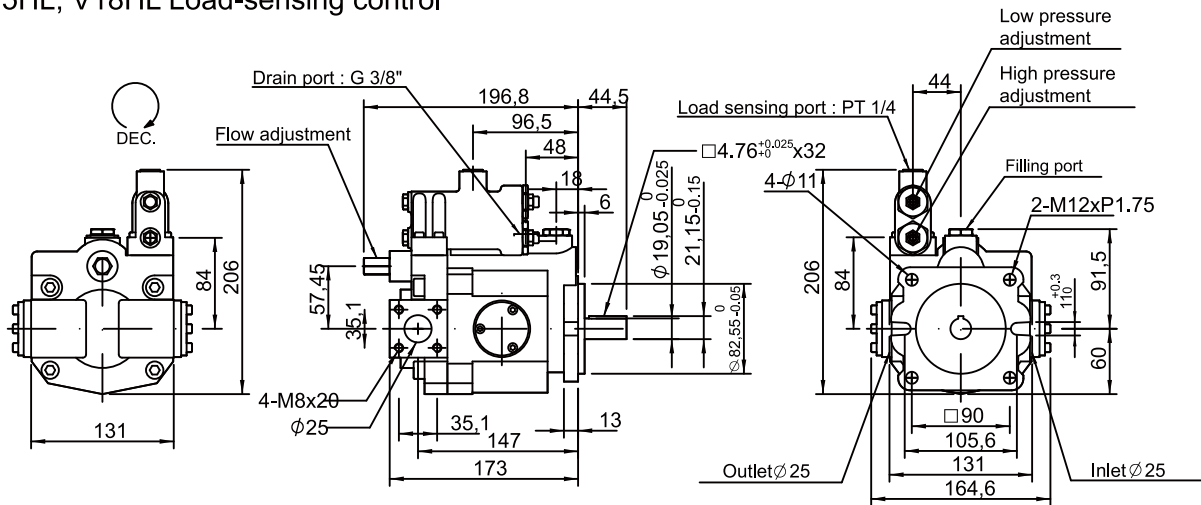
V15HL, V18HL Load-sensing control
