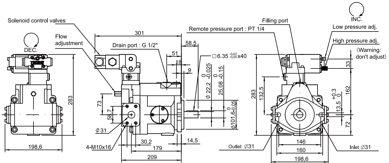
V38EG, V42EG Electric 2-stage pressure control + Remote
