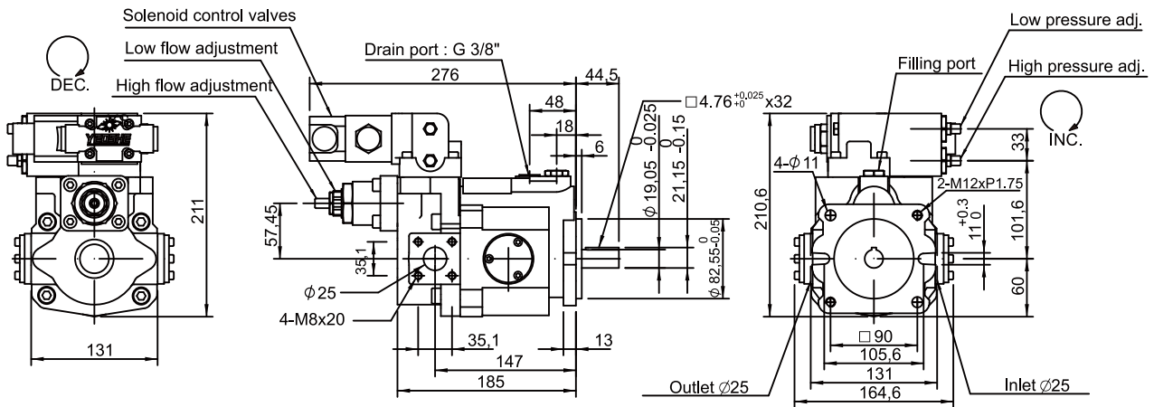
V15FG, V18FG Electric 2-stage pressure control & Flow control + Remote
